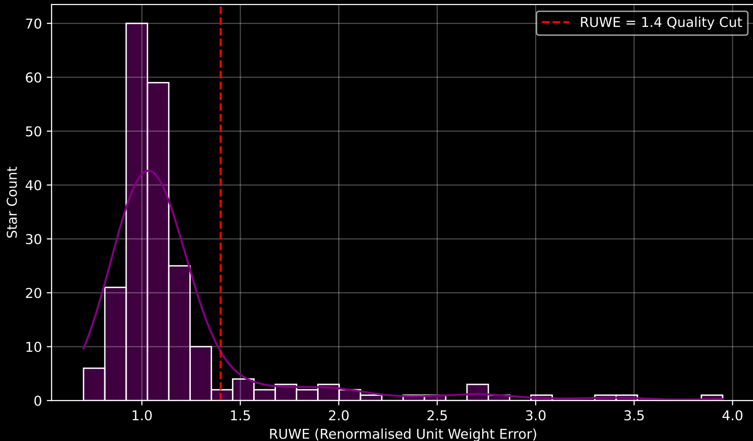
GAPOGEE DR17 Field [180-60] RUWE Distribution (n= 220)
