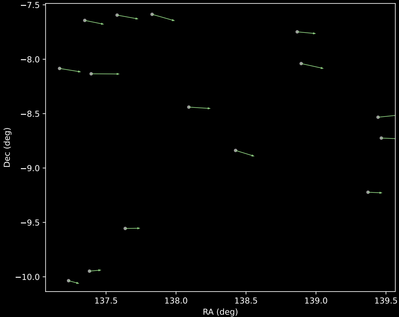
APOGEE DR17 Cluster 5 Proper Motion Vectors (n=15)
