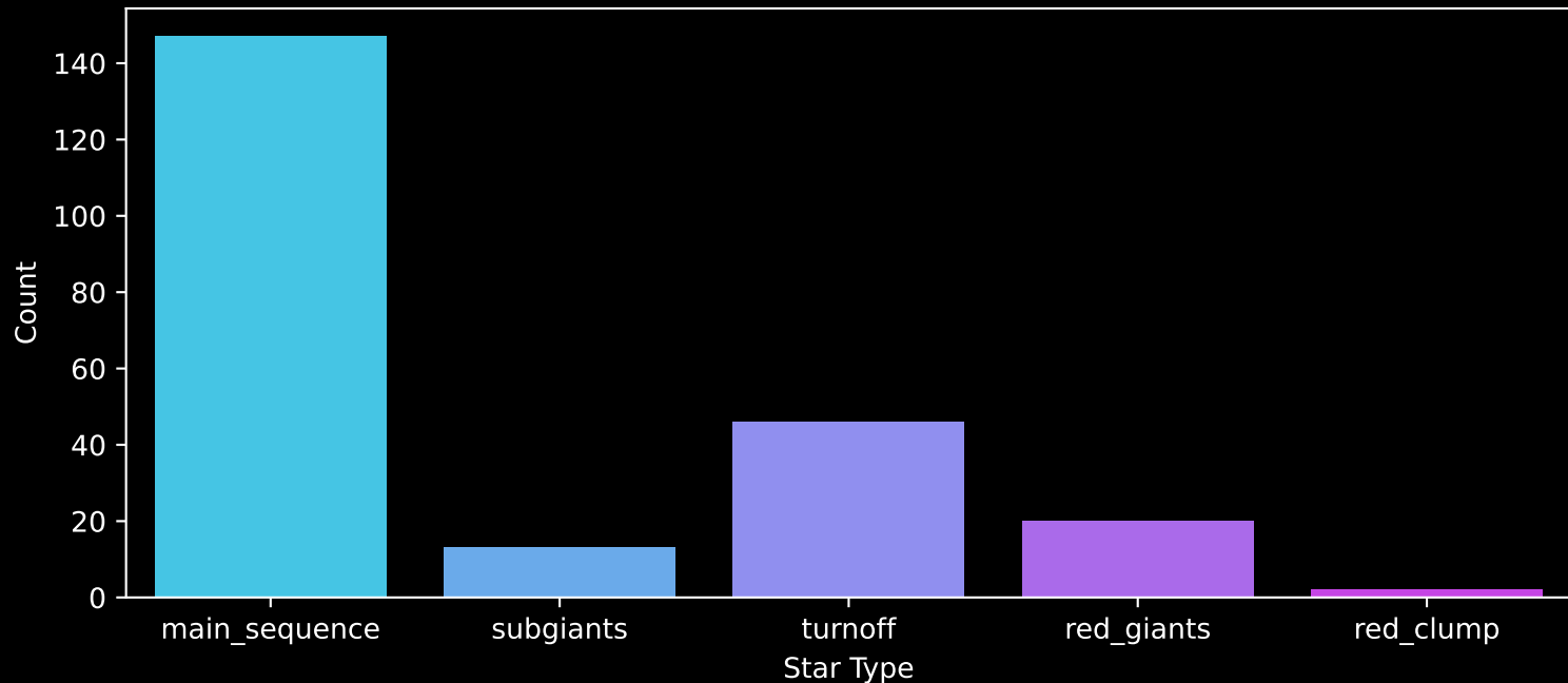
APOGEE DR17 Field: [180-60] Count plot of Star Type
