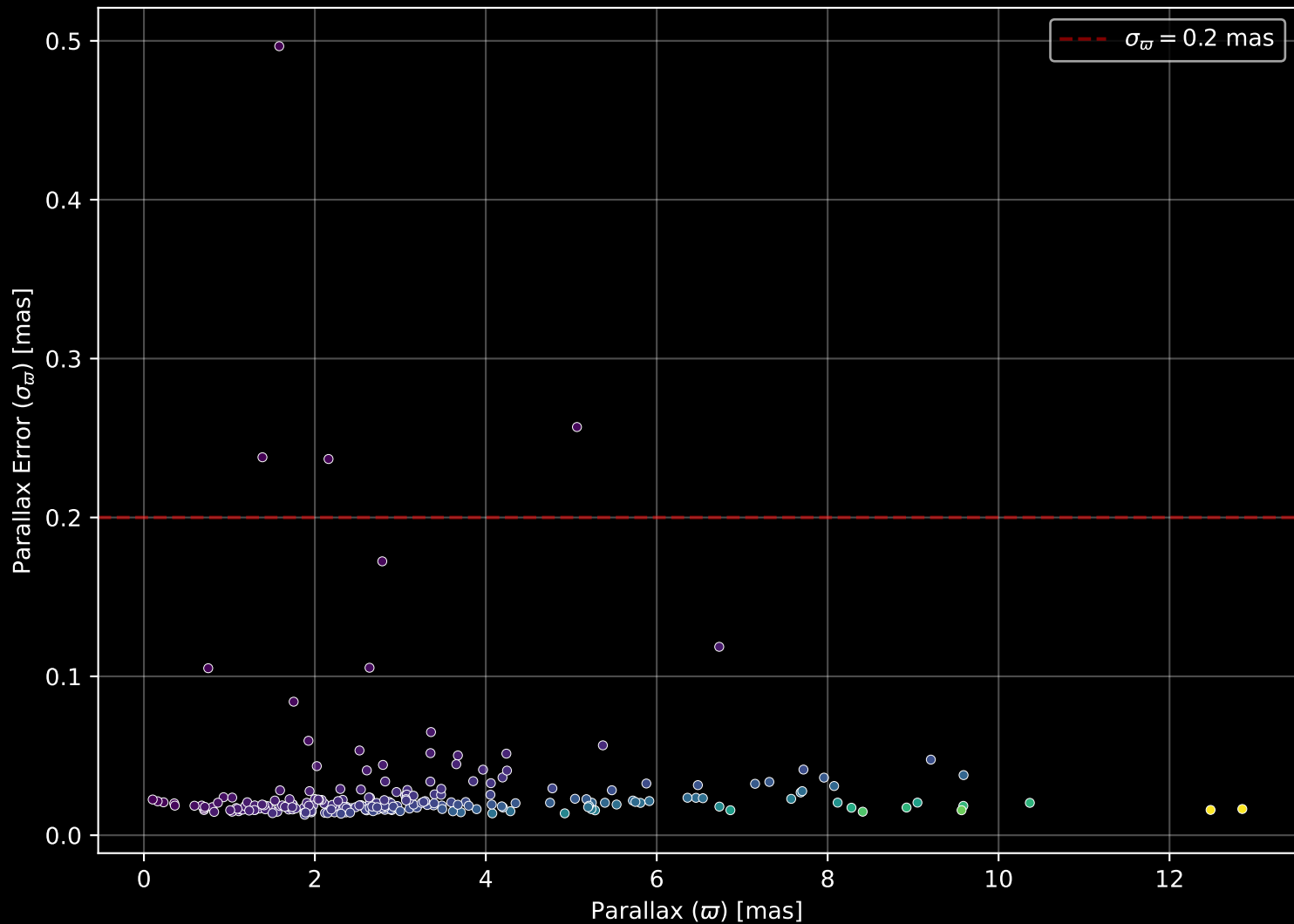
APOGEE DR17 Field: [180-60] Parallax Quality (n= 228)
