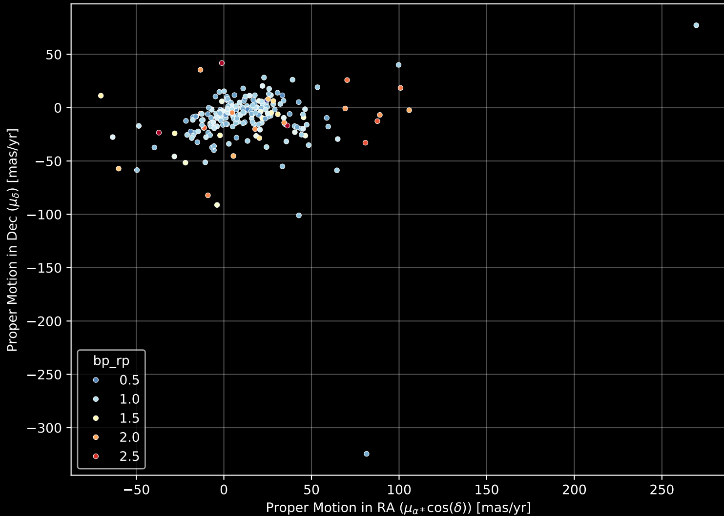
APOGEE DR17 Field: [180-60] Proper Motion Diagram (n= 228)
