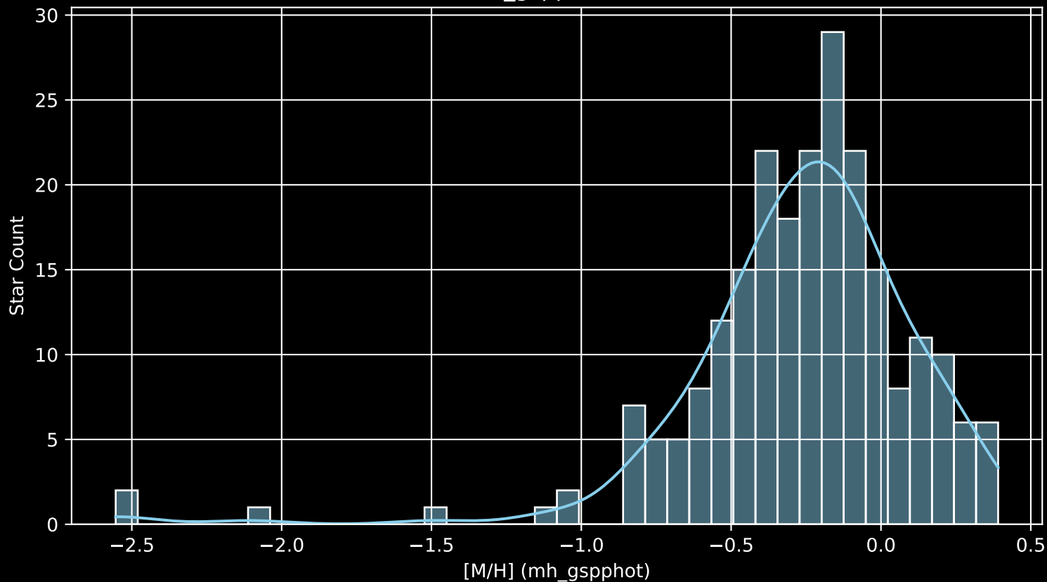
APOGEE DR17 Field: [180-60 [M/H] (mh_gspphot) (n= 228)
