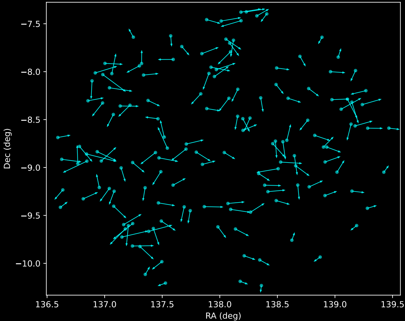
APOGEE DR17 Noise Stream Proper Motion Vectors (n=146)
